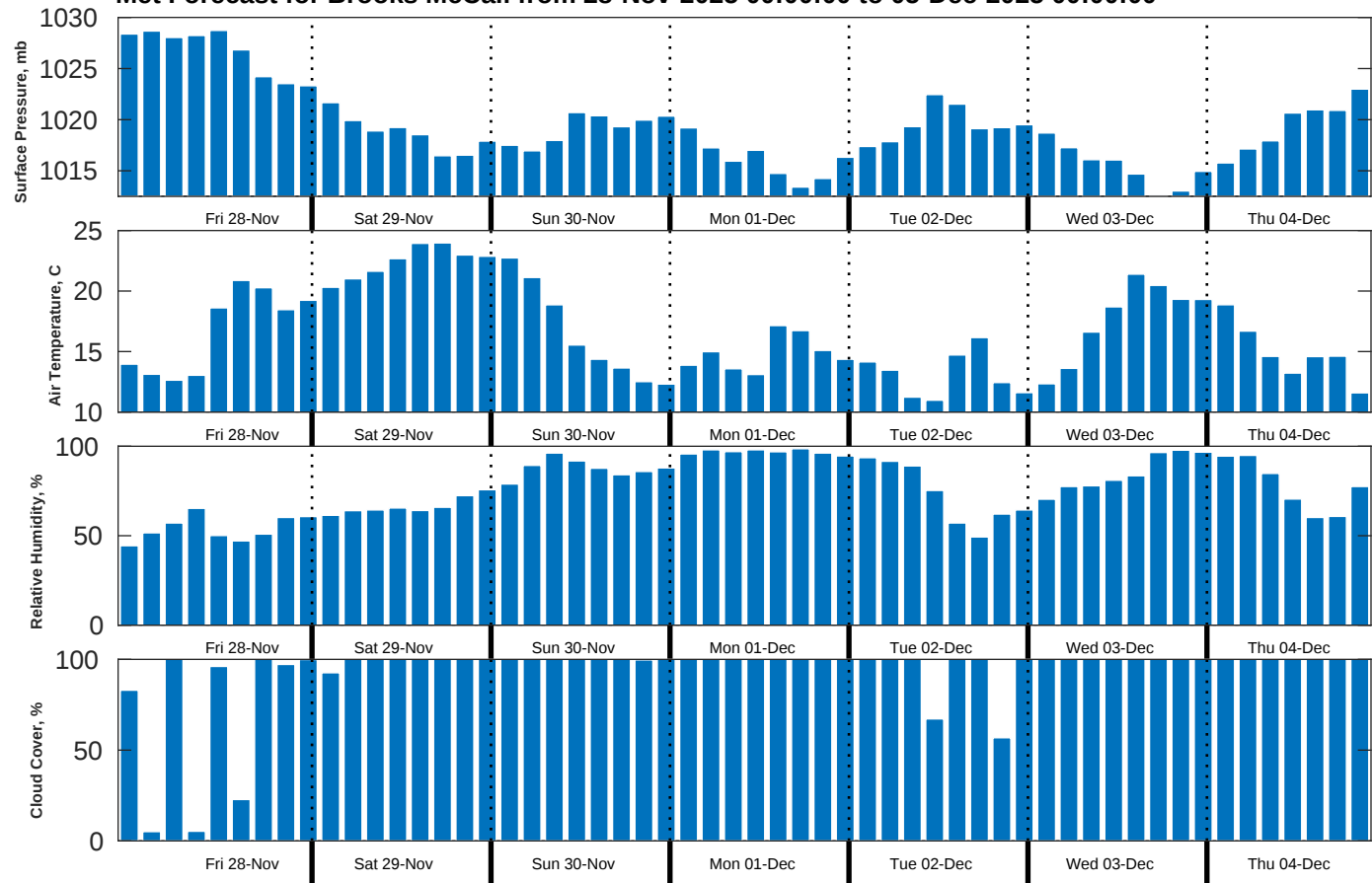
Met Forecast for Brooks McCall from 28-Nov-2025 00:00:00 to 05-Dec-2025 00:00:00
