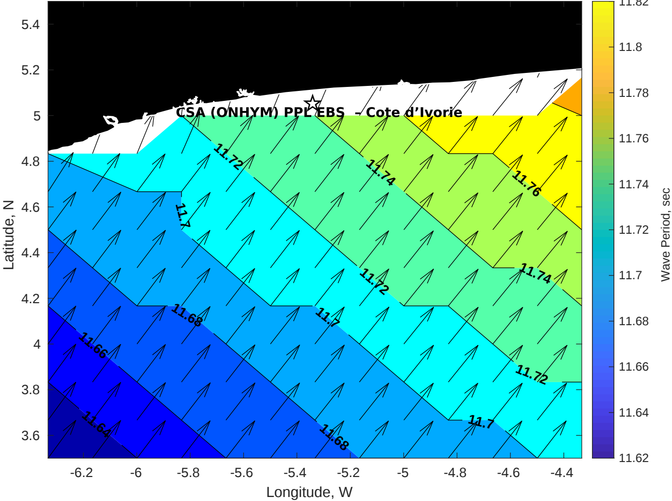
GFS Wave Period (sec) for CSA (ONHYM) PPL EBS - Cote d'Ivoire at 28-Nov-2025 09:00:00
