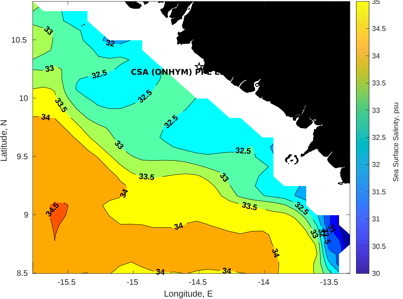
Surface Salinity for CSA (ONHYM) PPL EBS - Guinea at 27-Nov-2025 00:00:00
