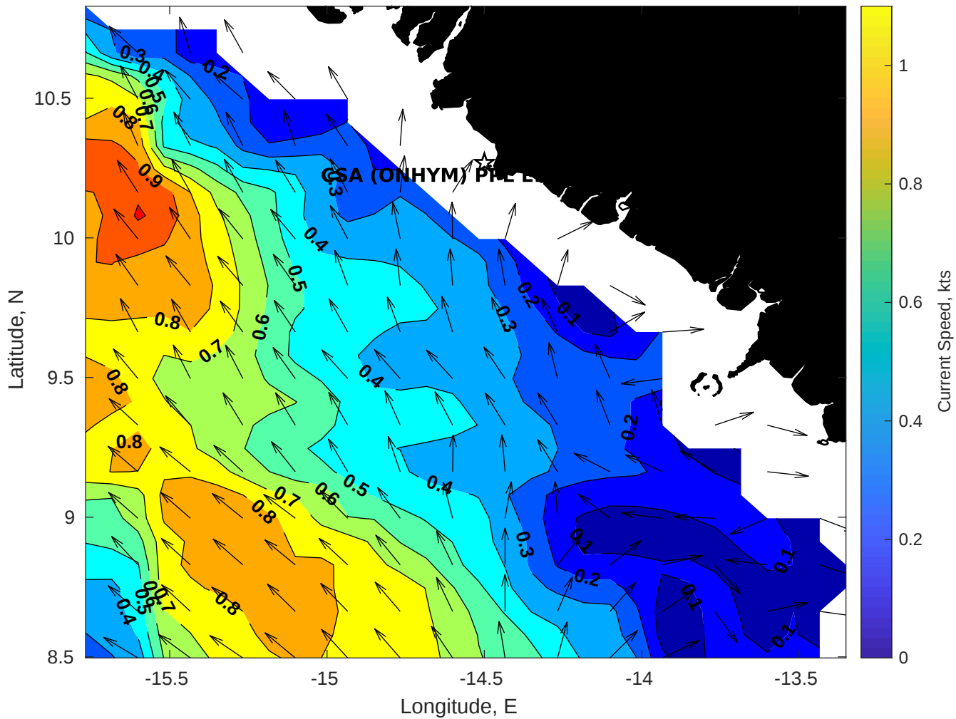
Surface Currents for CSA (ONHYM) PPL EBS - Guinea at 27-Nov-2025 00:00:00
