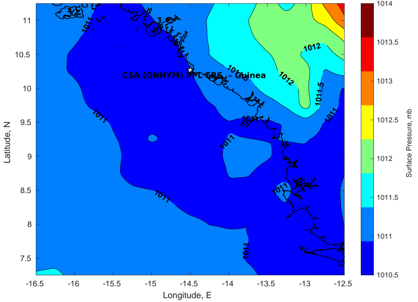
Surface Pressure (mb) for CSA (ONHYM) PPL EBS - Guinea at 29-Nov-2025 00:00:00
