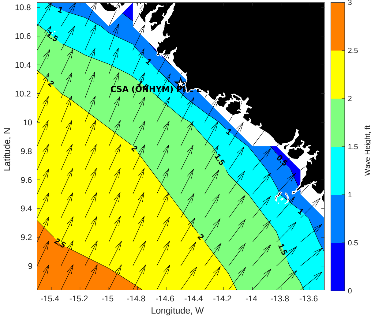
GFS Wave Height (ft) for CSA (ONHYM) PPL EBS - Guinea at 28-Nov-2025 09:00:00
