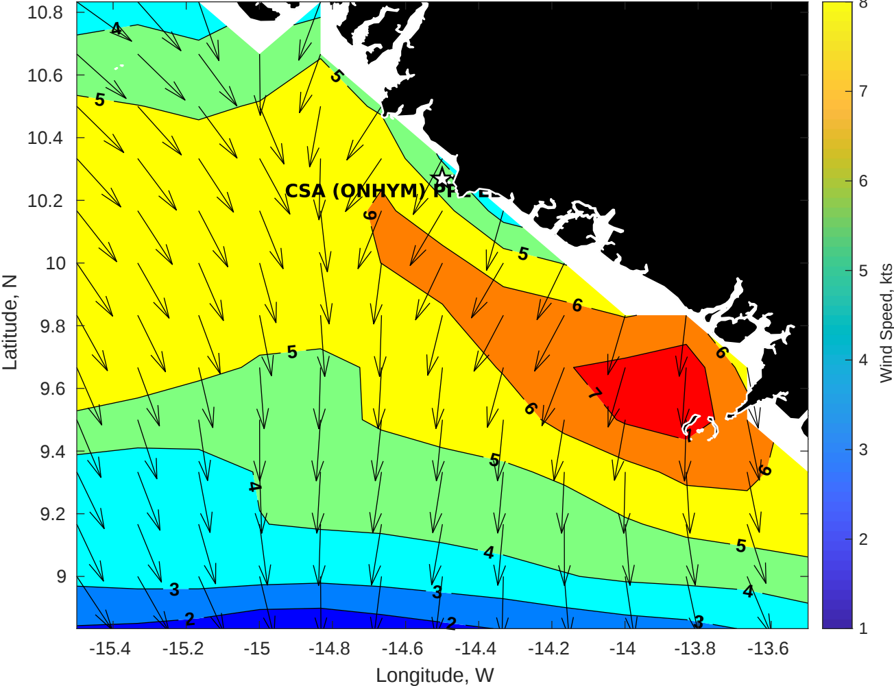
GFS Winds (kts) for CSA (ONHYM) PPL EBS - Guinea at 28-Nov-2025 09:00:00
