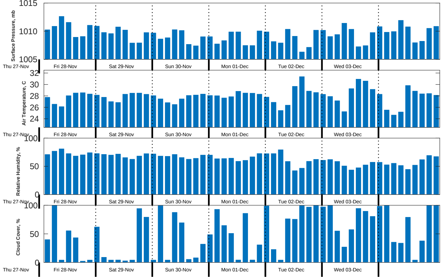
Met Forecast for CSA (ONHYM) PPL EBS - Guinea from 28-Nov-2025 00:00:00 to 05-Dec-2025 00:00:00
