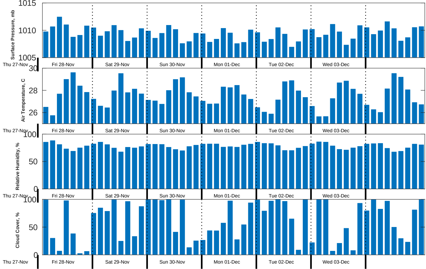
Met Forecast for CSA (ONHYM) PPL EBS - Liberia from 28-Nov-2025 00:00:00 to 05-Dec-2025 00:00:00
