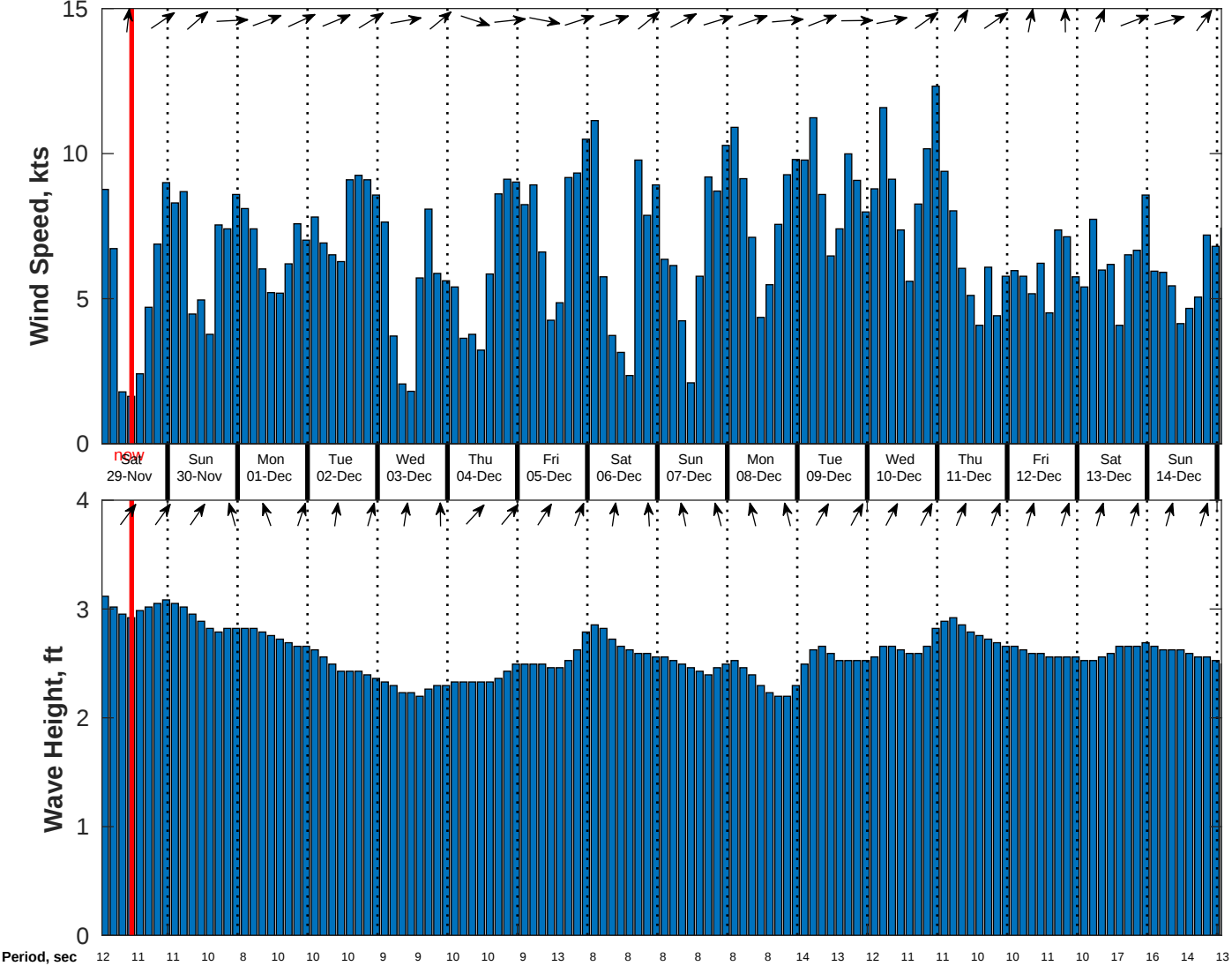
Wind & Wave Forecast for CSA (ONHYM) PPL EBS - Liberia from 28-Nov-2025 01:00:00 to 14-Dec-2025 01:00:00
