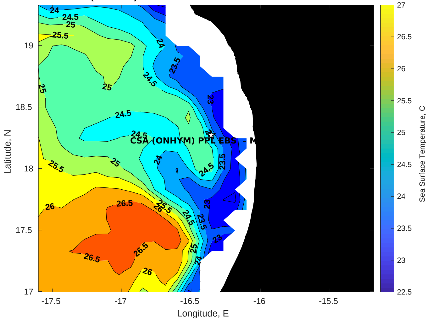
SST for CSA (ONHYM) PPL EBS - Mauritania at 27-Nov-2025 00:00:00
