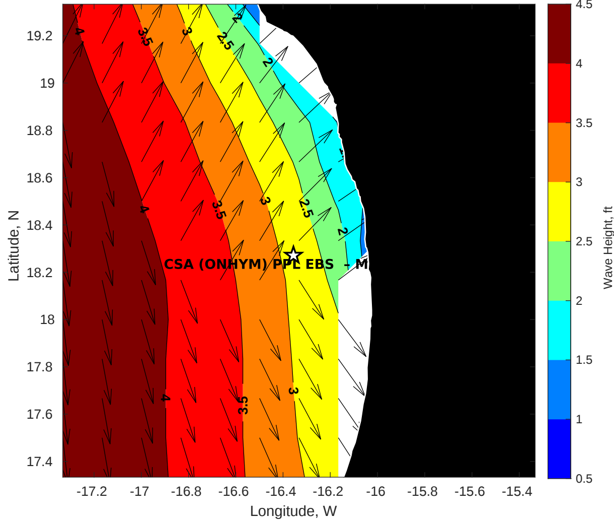
GFS Wave Height (ft) for CSA (ONHYM) PPL EBS - Mauritania at 28-Nov-2025 09:00:00
