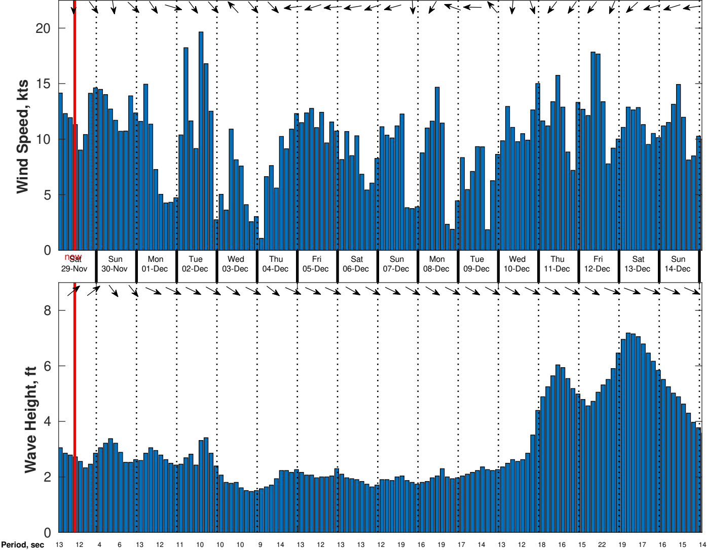
Wind & Wave Forecast for CSA (ONHYM) PPL EBS - Mauritania from 28-Nov-2025 01:00:00 to 14-Dec-2025 01:00:00
