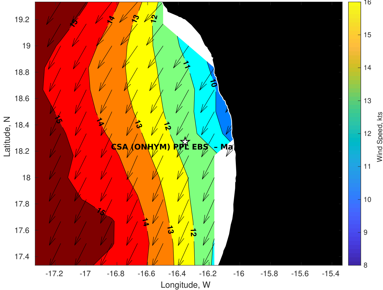
GFS Winds (kts) for CSA (ONHYM) PPL EBS - Mauritania at 28-Nov-2025 09:00:00
