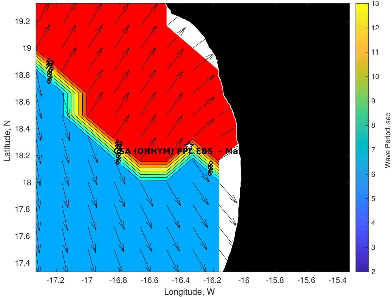
GFS Wave Period (sec) for CSA (ONHYM) PPL EBS - Mauritania at 28-Nov-2025 09:00:00
