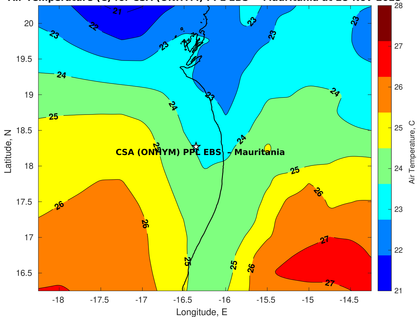
Air Temperature (C) for CSA (ONHYM) PPL EBS - Mauritania at 28-Nov-2025
