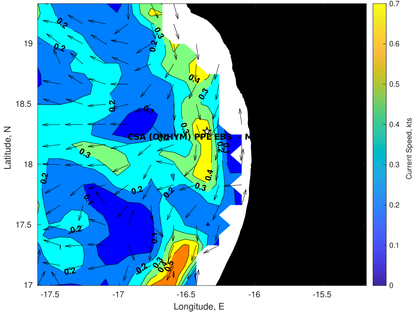
Surface Currents for CSA (ONHYM) PPL EBS - Mauritania at 27-Nov-2025 00:00:00
