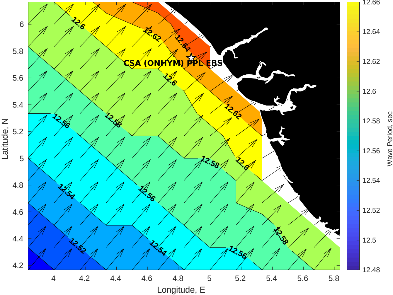
GFS Wave Period (sec) for CSA (ONHYM) PPL EBS - Nigeria at 28-Nov-2025 09:00:00
