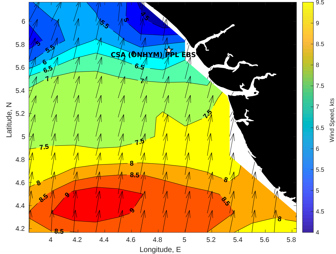
GFS Winds (kts) for CSA (ONHYM) PPL EBS - Nigeria at 28-Nov-2025 09:00:00
