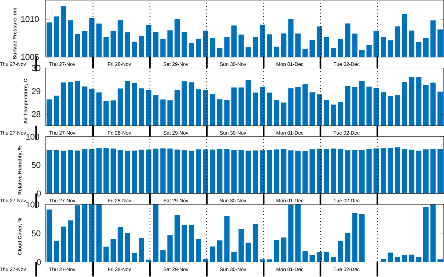
Met Forecast for CSA (ONHYM) PPL EBS - Nigeria from 28-Nov-2025 00:00:00 to 05-Dec-2025 00:00:00
