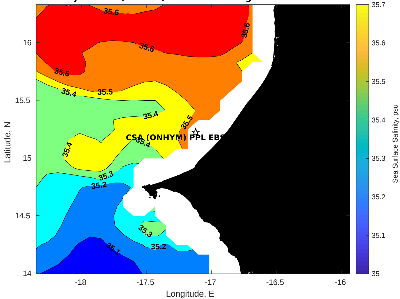
Surface Salinity for CSA (ONHYM) PPL EBS - Senegal at 27-Nov-2025 00:00:00
