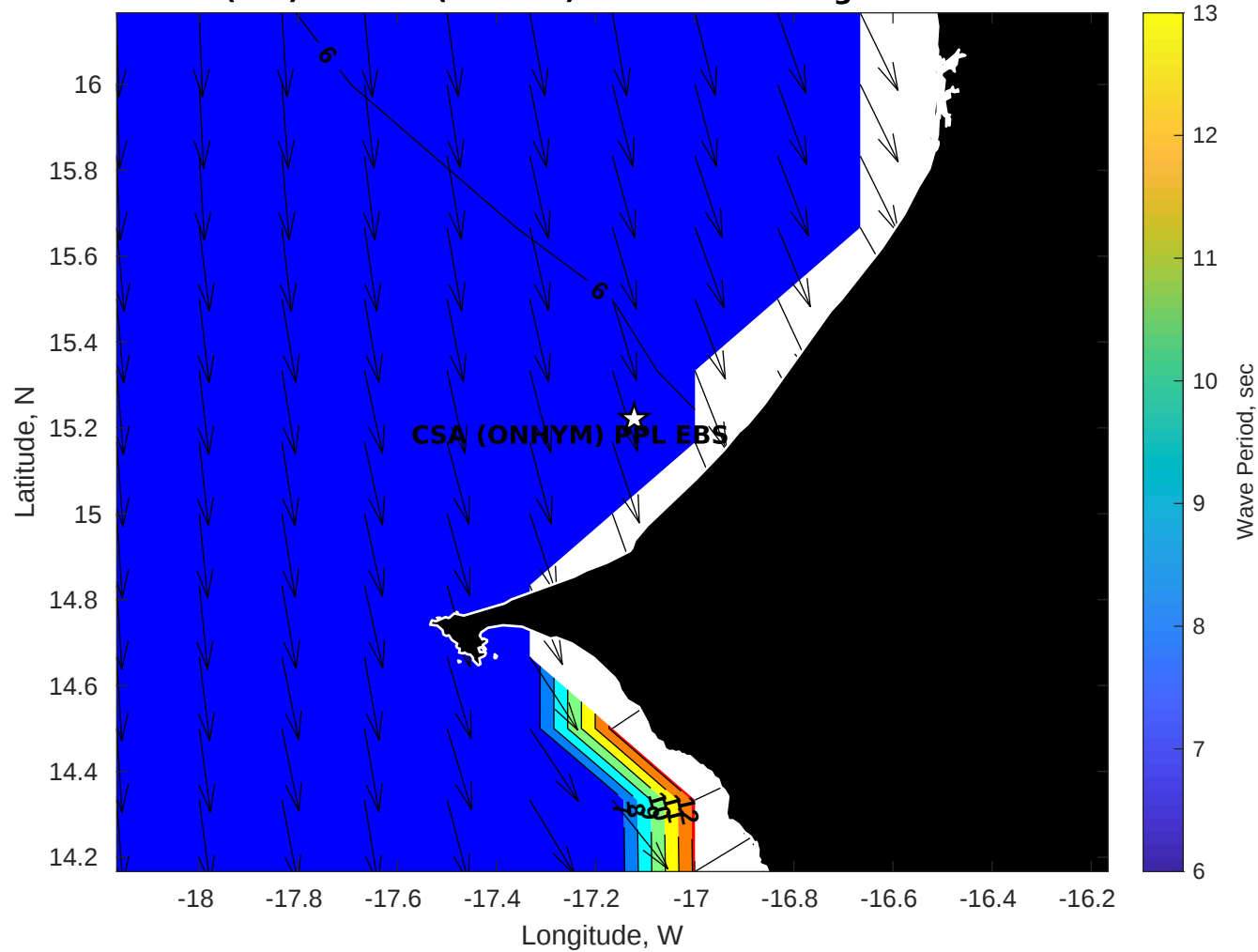
GFS Wave Period (sec) for CSA (ONHYM) PPL EBS - Senegal at 28-Nov-2025 09:00:00
