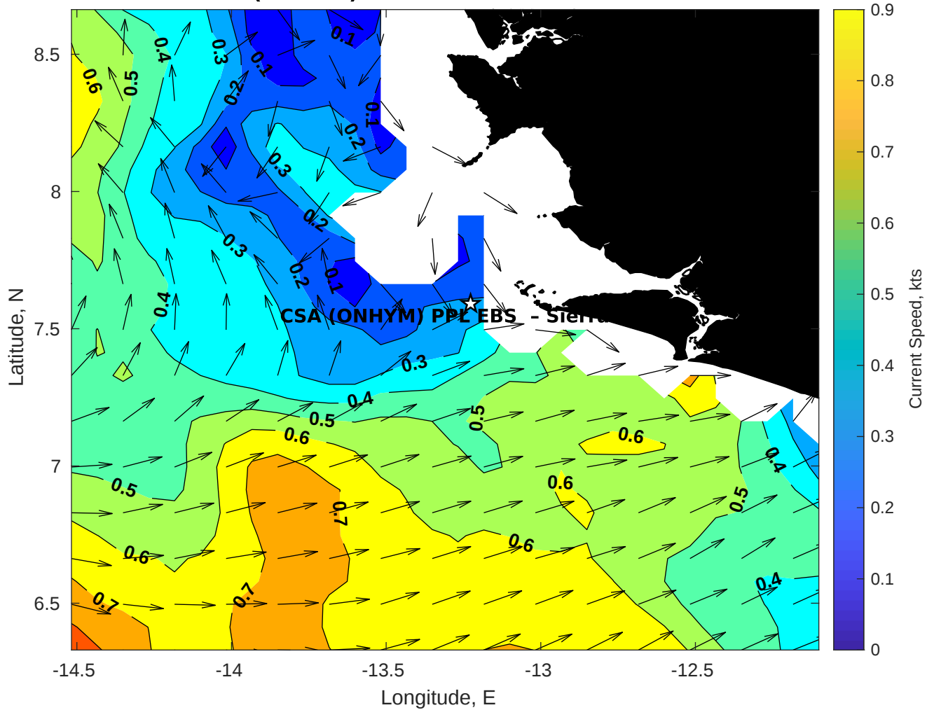
Surface Currents for CSA (ONHYM) PPL EBS - Sierra Leone at 27-Nov-2025 00:00:00
