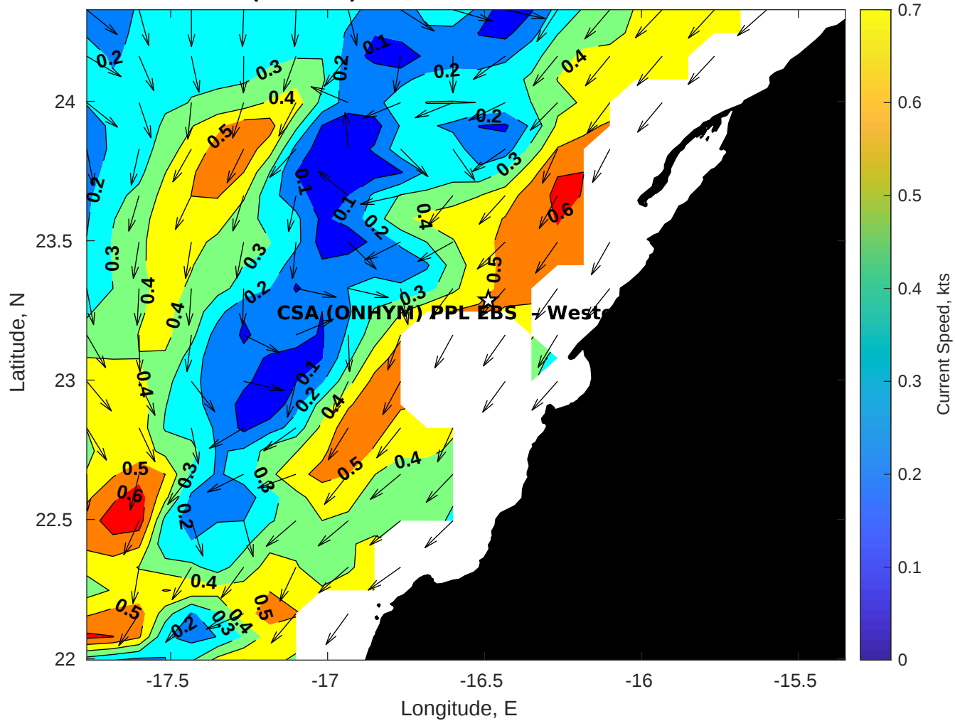
Surface Currents for CSA (ONHYM) PPL EBS - Western Sahara at 27-Nov-2025 00:00:00
