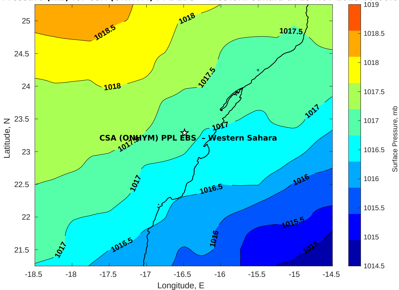
Surface Pressure (mb) for CSA (ONHYM) PPL EBS - Western Sahara at 29-Nov-2025 00:00:00
