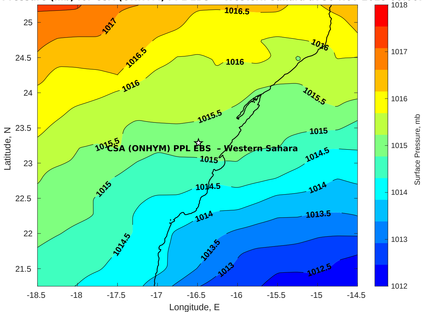
Surface Pressure (mb) for CSA (ONHYM) PPL EBS - Western Sahara at 30-Nov-2025 00:00:00
