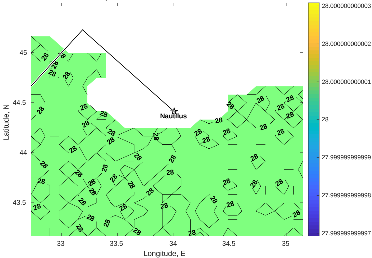
Surface Salinity for Nautilus at 27-Nov-2025 00:00:00
