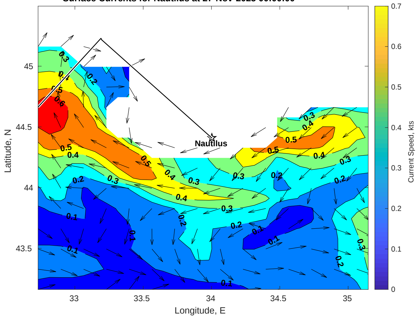
Surface Currents for Nautilus at 27-Nov-2025 00:00:00
