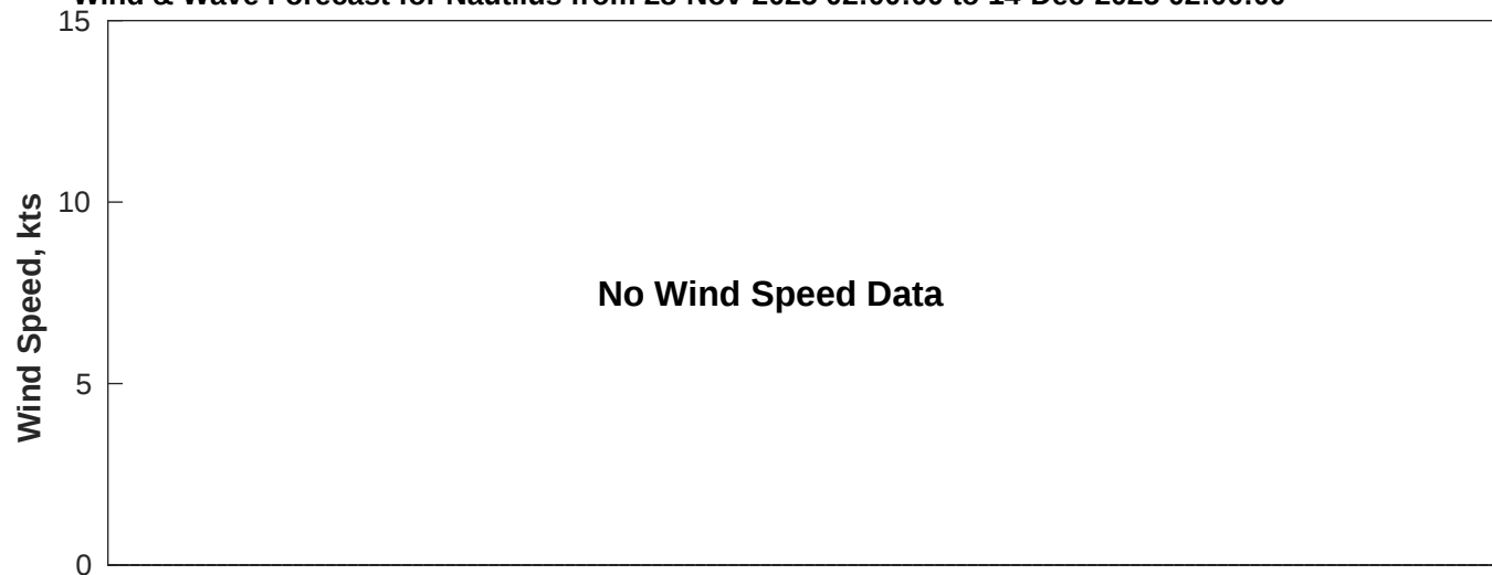
Wind & Wave Forecast for Nautilus from 28-Nov-2025 02:00:00 to 14-Dec-2025 02:00:00
