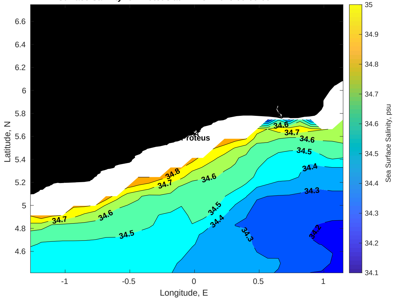
Surface Salinity for Proteus at 27-Nov-2025 00:00:00
