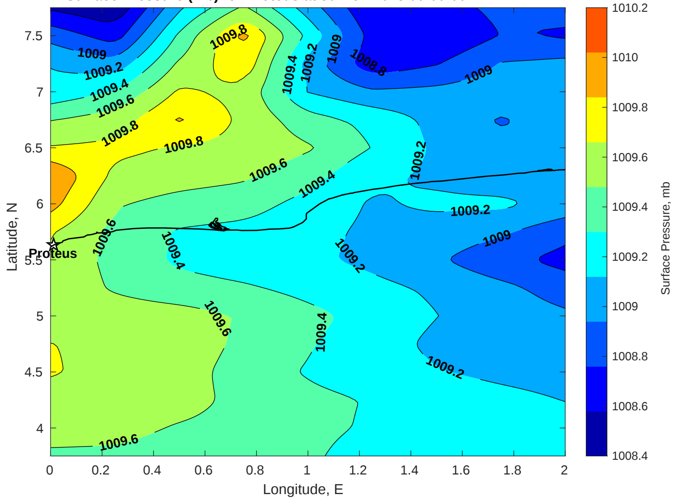
Surface Pressure (mb) for Proteus at 30-Nov-2025 00:00:00
