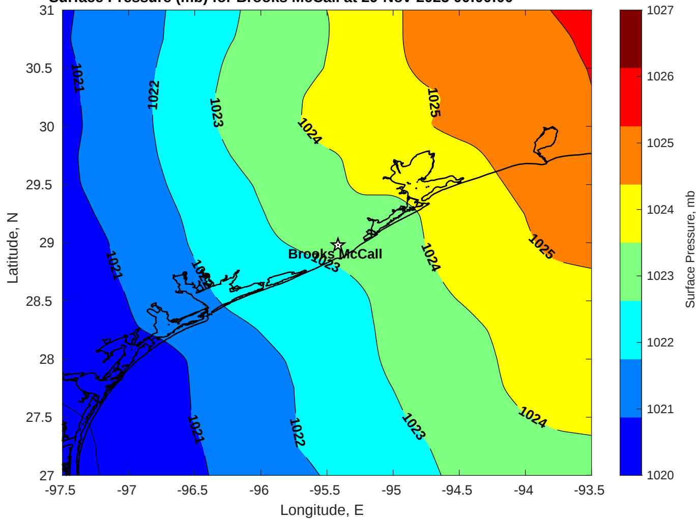
Surface Pressure (mb) for Brooks McCall at 29-Nov-2025 00:00:00
