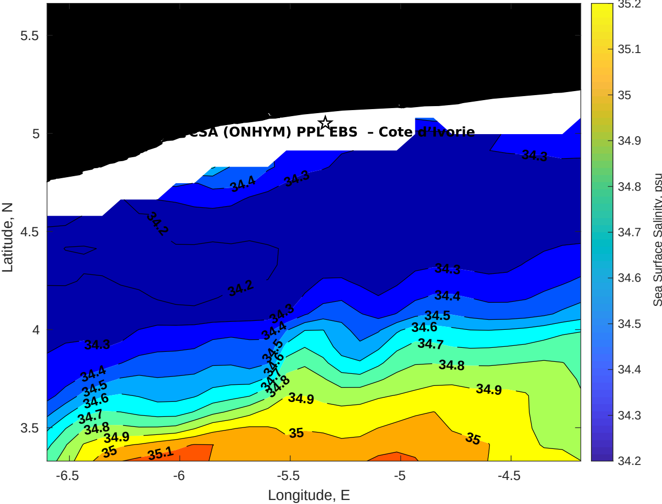
Surface Salinity for CSA (ONHYM) PPL EBS - Cote d'Ivoire at 28-Nov-2025 00:00:00
