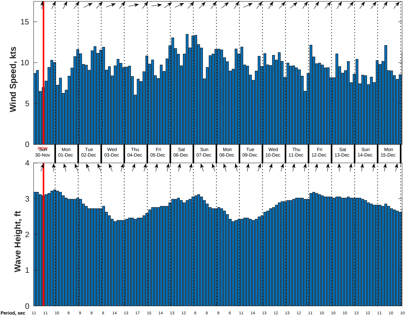
Wind & Wave Forecast for CSA (ONHYM) PPL EBS - Cote d'Ivoire from 29-Nov-2025 01:00:00 to 15-Dec-2025 01:00:00
