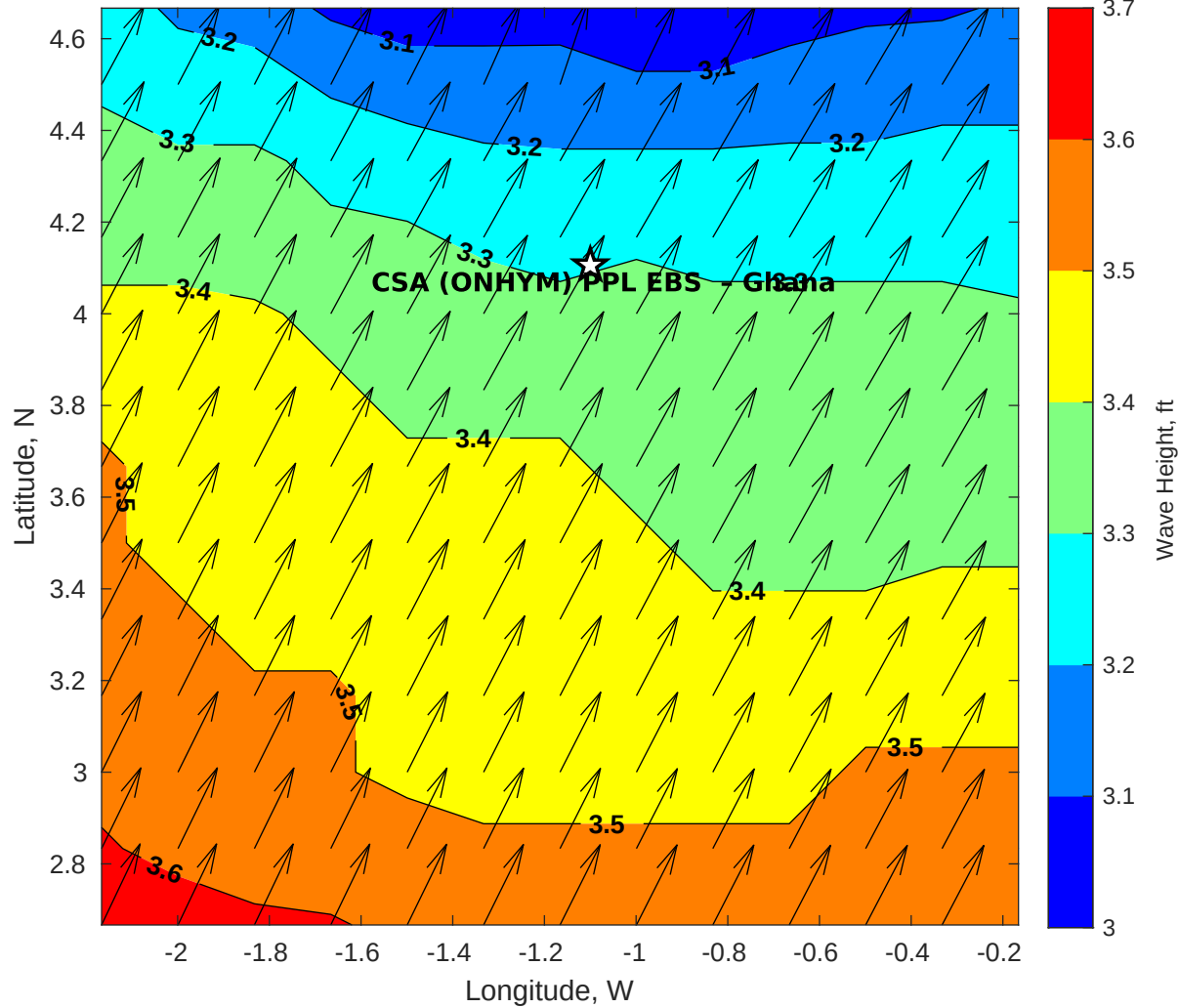
GFS Wave Height (ft) for CSA (ONHYM) PPL EBS - Ghana at 29-Nov-2025 09:00:00
