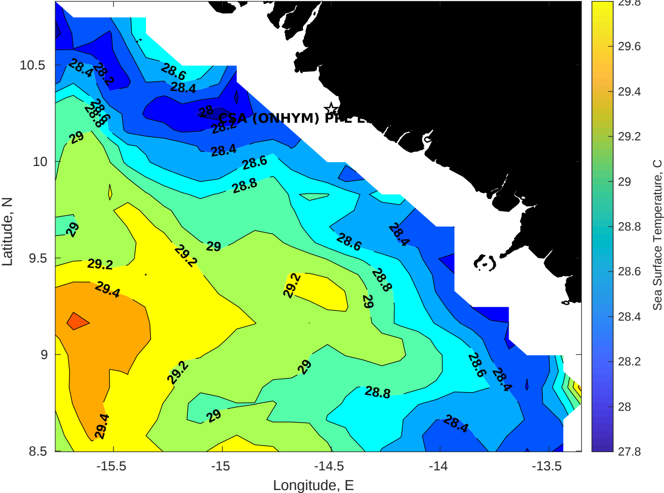
SST for CSA (ONHYM) PPL EBS - Guinea at 28-Nov-2025 00:00:00
