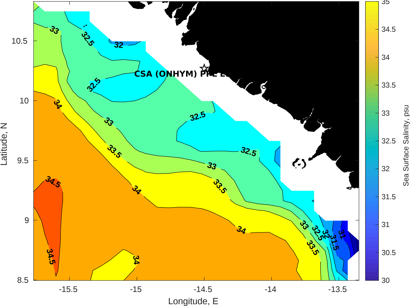
Surface Salinity for CSA (ONHYM) PPL EBS - Guinea at 28-Nov-2025 00:00:00
