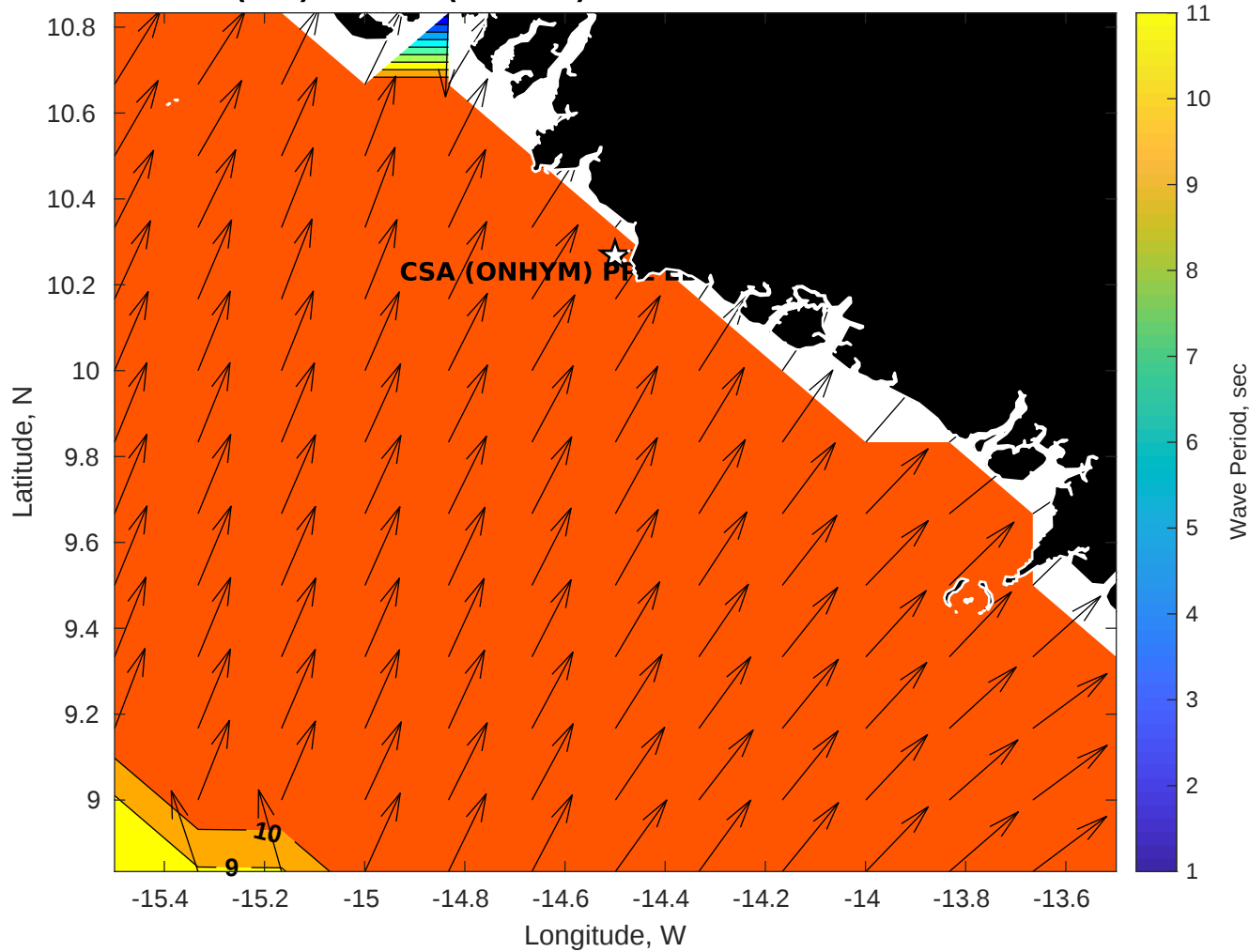
GFS Wave Period (sec) for CSA (ONHYM) PPL EBS - Guinea at 29-Nov-2025 09:00:00
