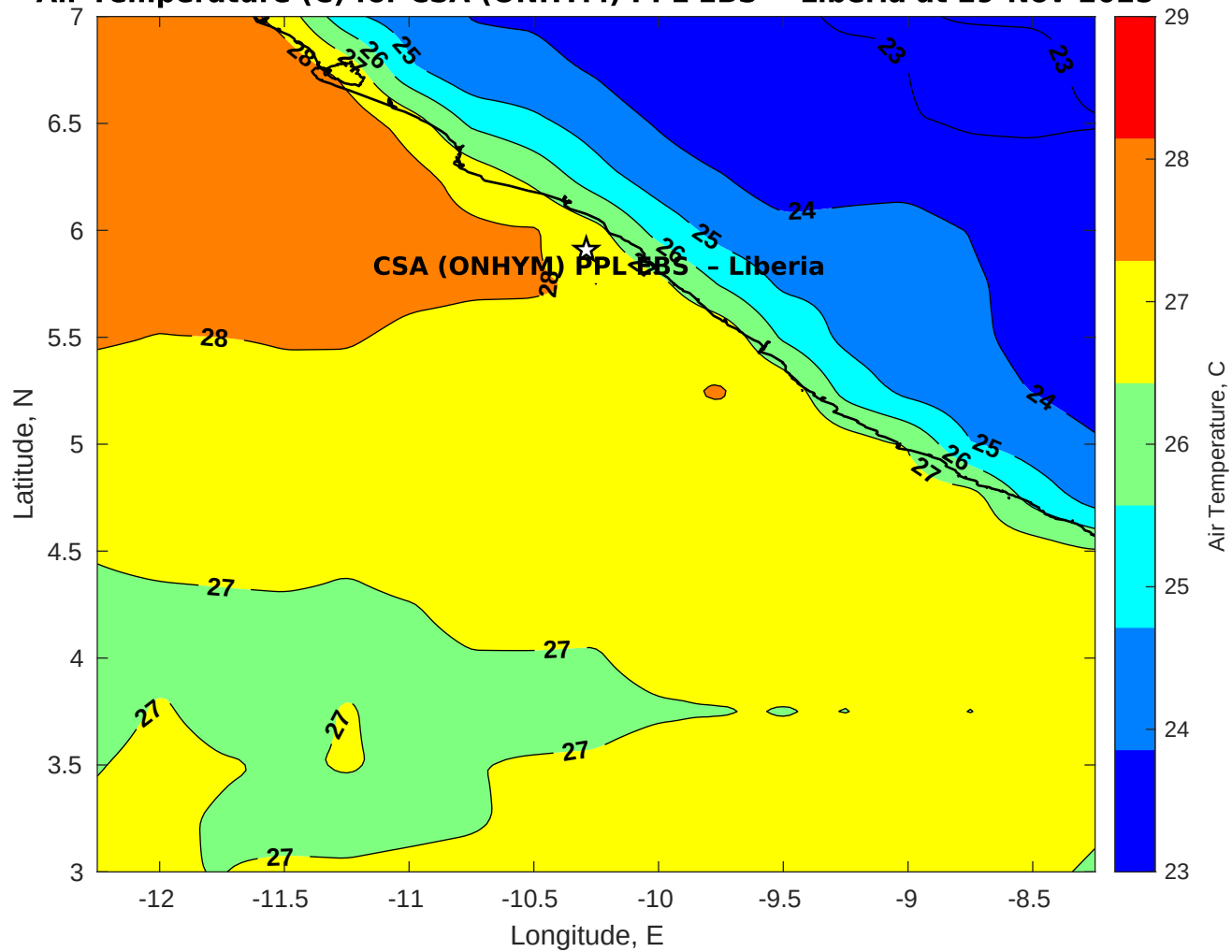
Air Temperature (C) for CSA (ONHYM) PPL EBS - Liberia at 29-Nov-2025
