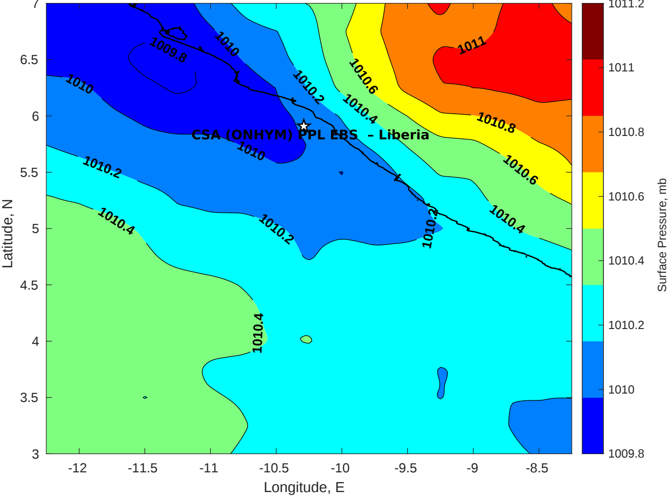
Surface Pressure (mb) for CSA (ONHYM) PPL EBS - Liberia at 30-Nov-2025 00:00:00
