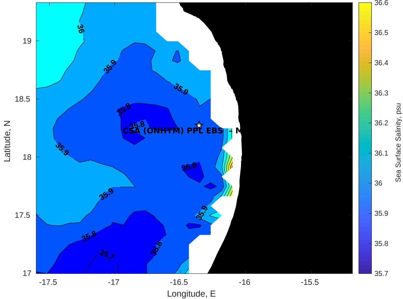
Surface Salinity for CSA (ONHYM) PPL EBS - Mauritania at 28-Nov-2025 00:00:00
