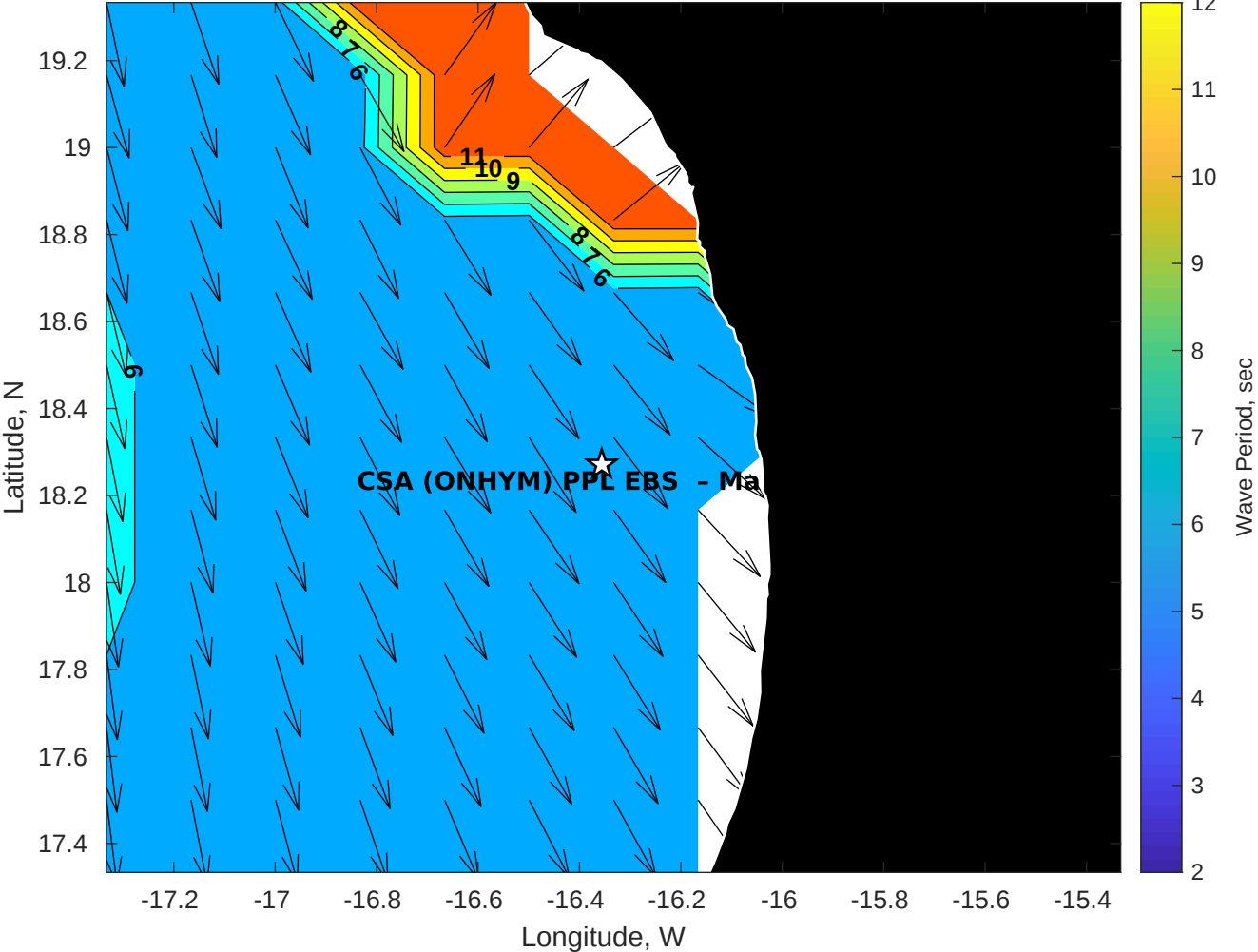
GFS Wave Period (sec) for CSA (ONHYM) PPL EBS - Mauritania at 29-Nov-2025 09:00:00
