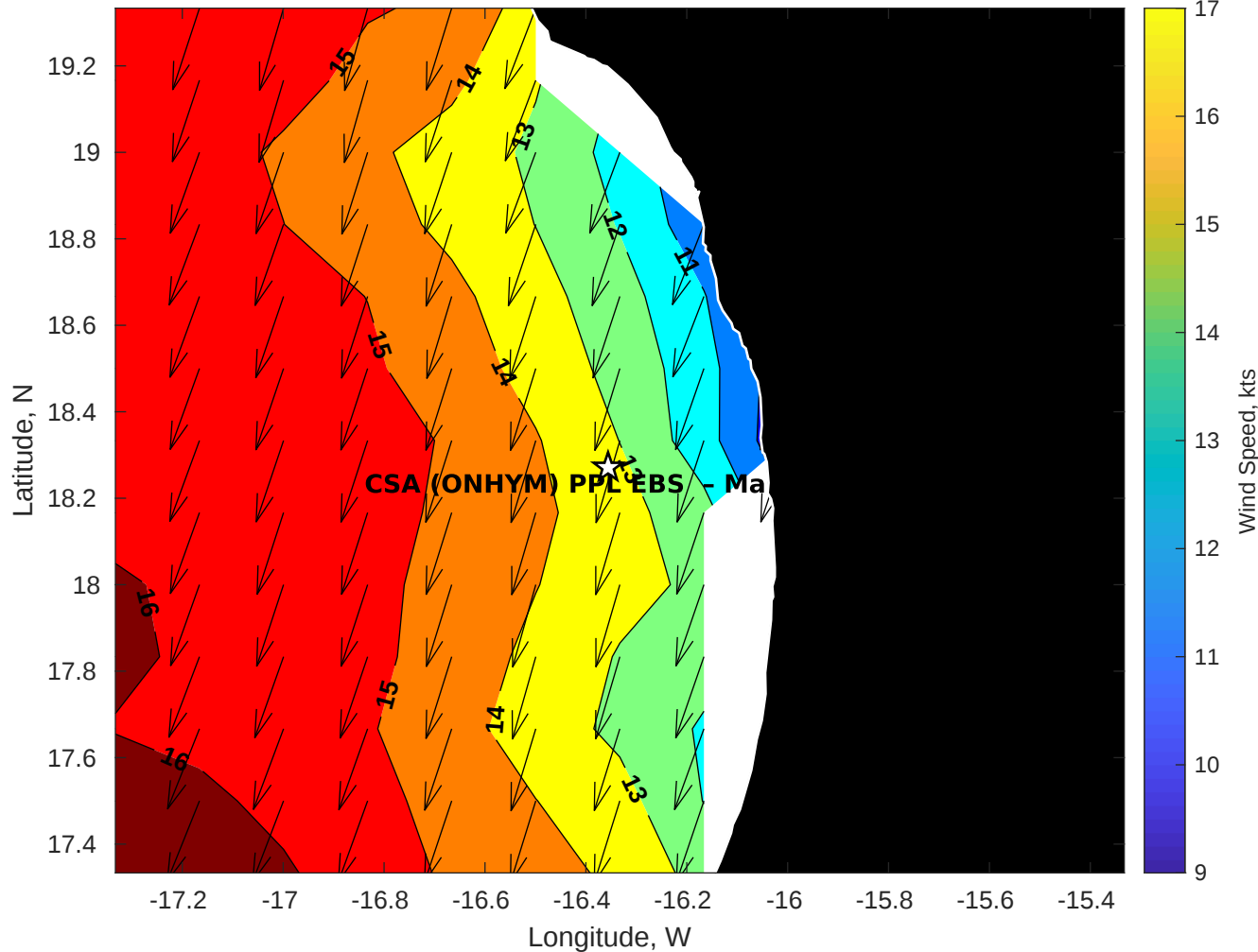
GFS Winds (kts) for CSA (ONHYM) PPL EBS - Mauritania at 29-Nov-2025 09:00:00
