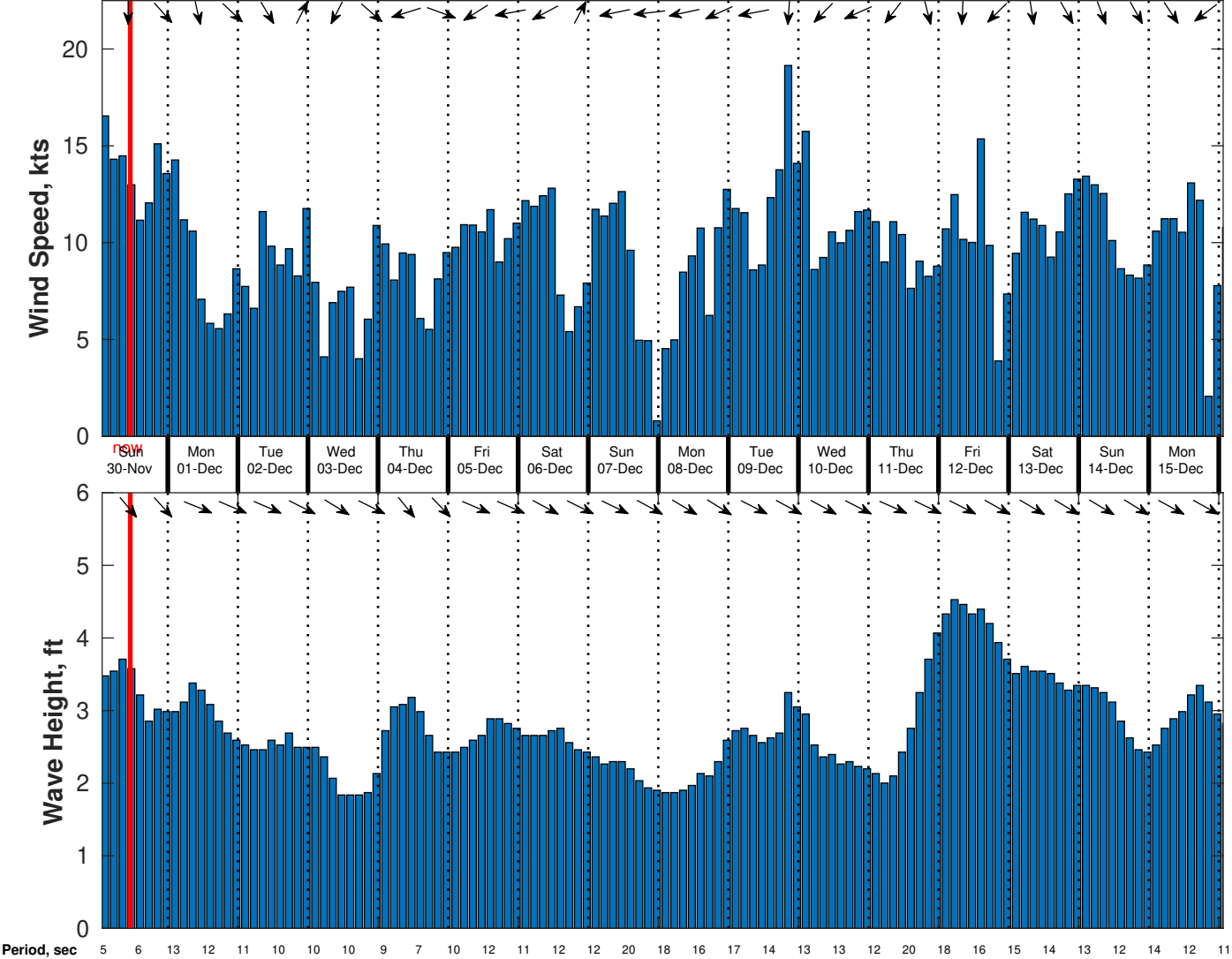
Wind & Wave Forecast for CSA (ONHYM) PPL EBS - Mauritania from 29-Nov-2025 01:00:00 to 15-Dec-2025 01:00:00
