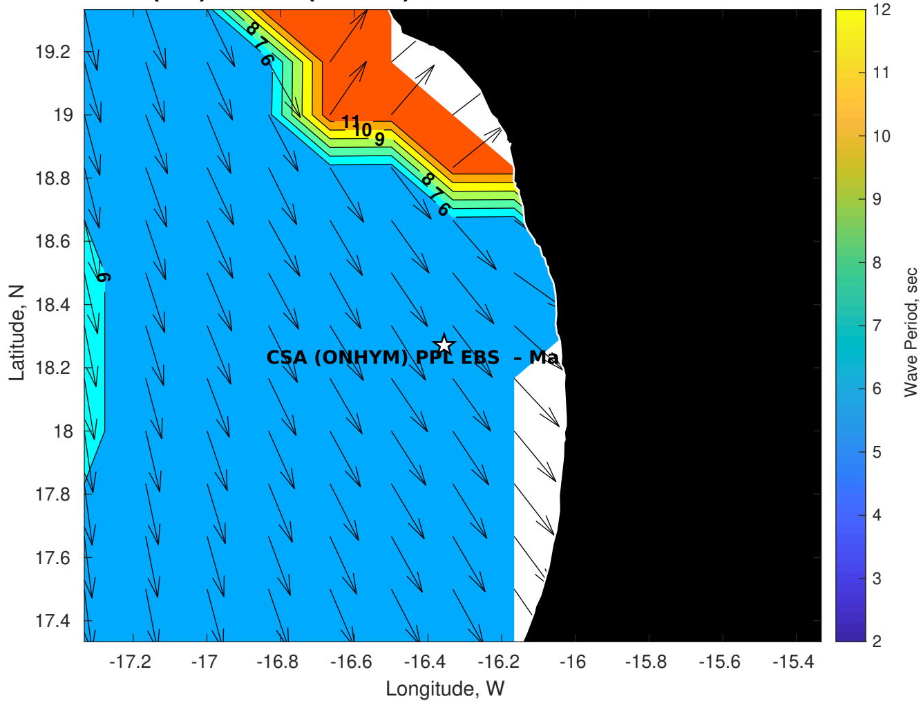
GFS Wave Period (sec) for CSA (ONHYM) PPL EBS - Mauritania at 29-Nov-2025 09:00:00
