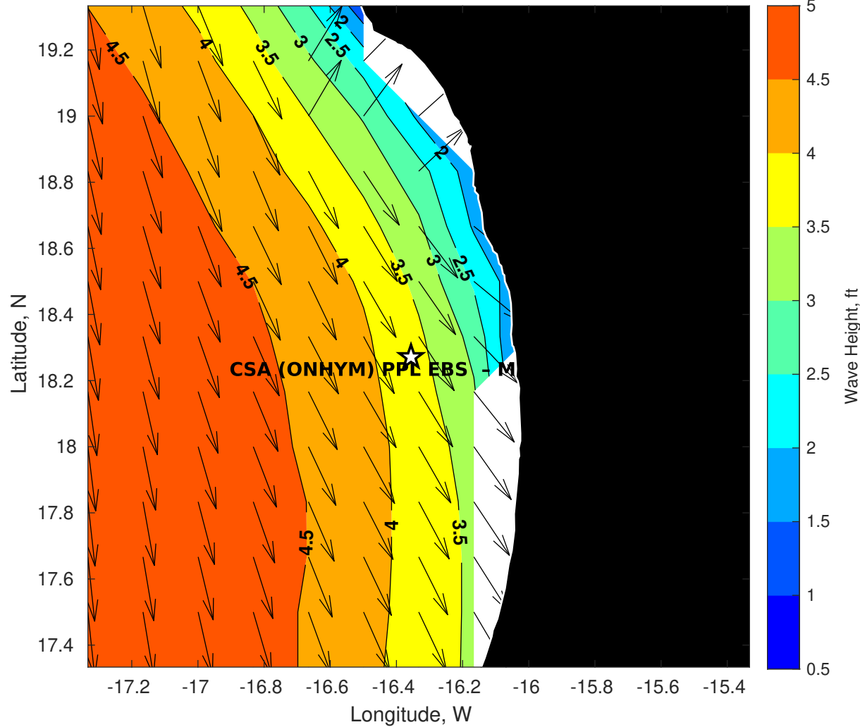
GFS Wave Height (ft) for CSA (ONHYM) PPL EBS - Mauritania at 29-Nov-2025 09:00:00
