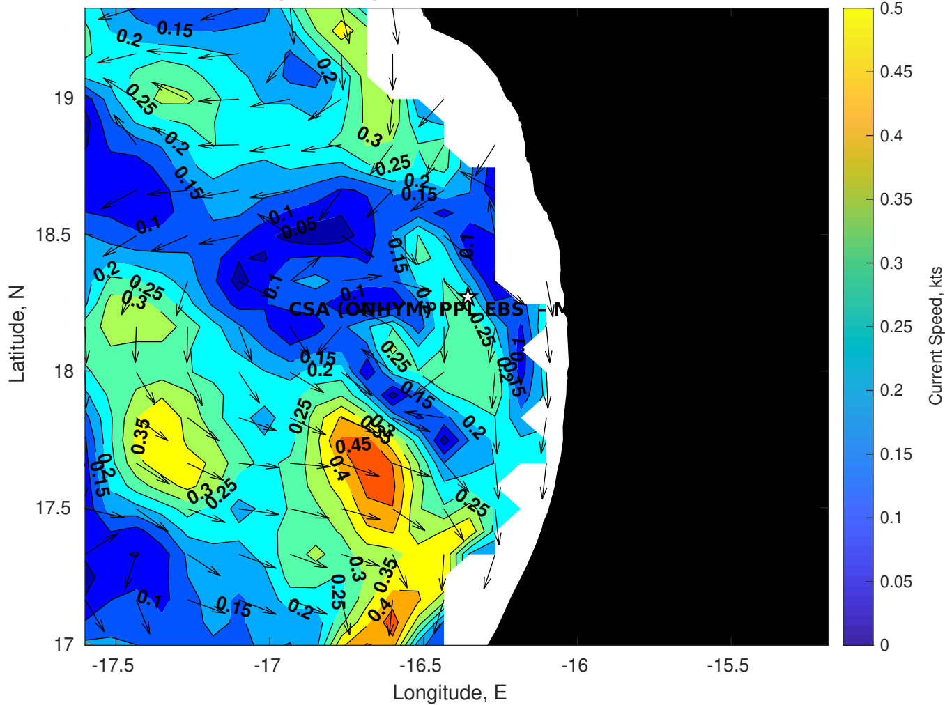
Surface Currents for CSA (ONHYM) PPL EBS - Mauritania at 28-Nov-2025 00:00:00
