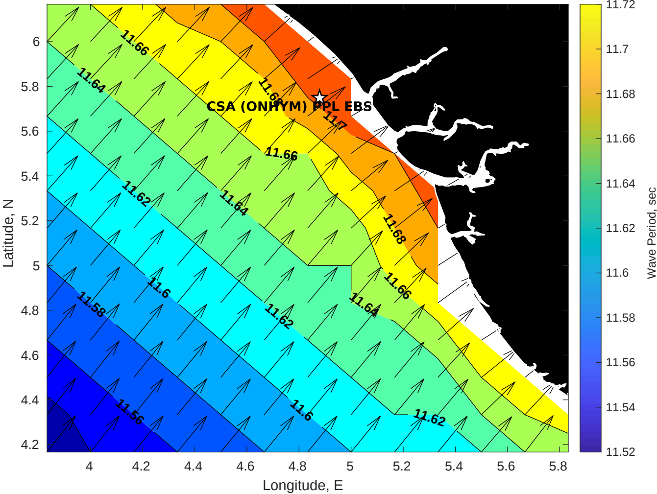
GFS Wave Period (sec) for CSA (ONHYM) PPL EBS - Nigeria at 29-Nov-2025 09:00:00
