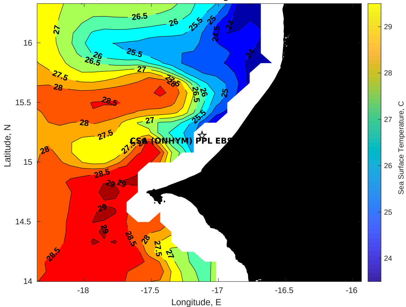
SST for CSA (ONHYM) PPL EBS - Senegal at 28-Nov-2025 00:00:00
