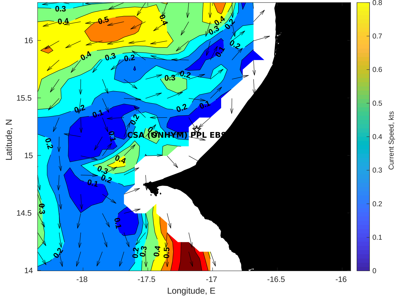
Surface Currents for CSA (ONHYM) PPL EBS - Senegal at 28-Nov-2025 00:00:00
