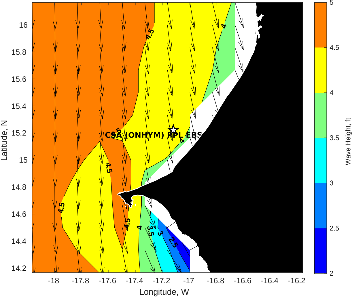
GFS Wave Height (ft) for CSA (ONHYM) PPL EBS - Senegal at 29-Nov-2025 09:00:00
