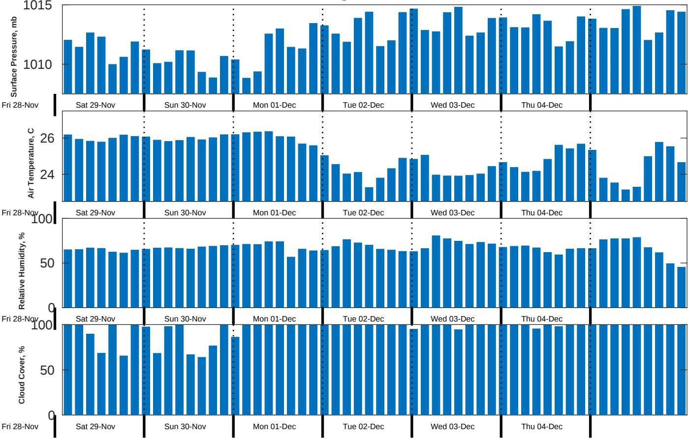
Met Forecast for CSA (ONHYM) PPL EBS - Senegal from 29-Nov-2025 00:00:00 to 06-Dec-2025 00:00:00
