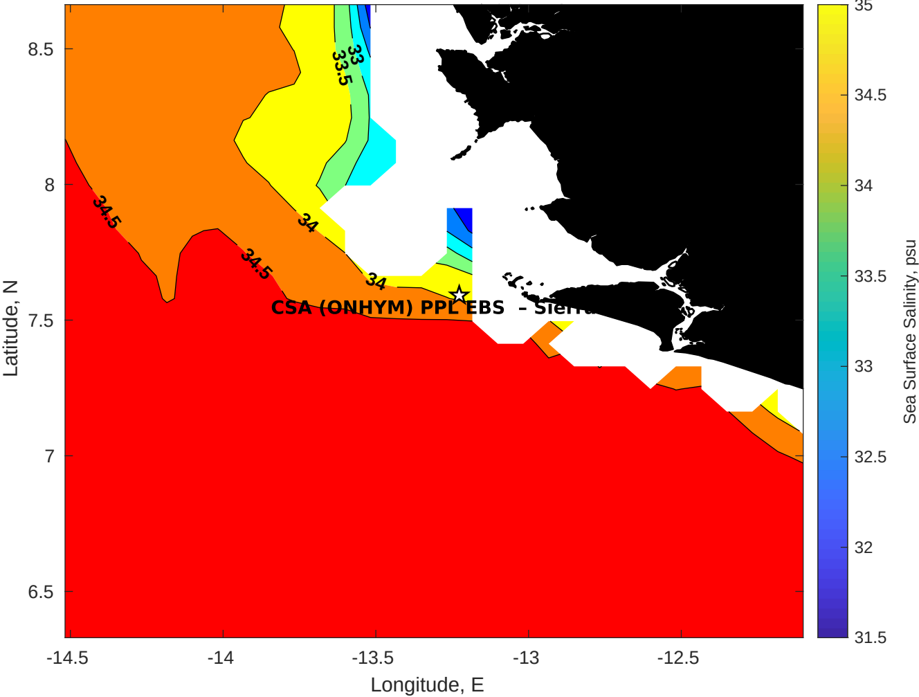
Surface Salinity for CSA (ONHYM) PPL EBS - Sierra Leone at 28-Nov-2025 00:00:00
