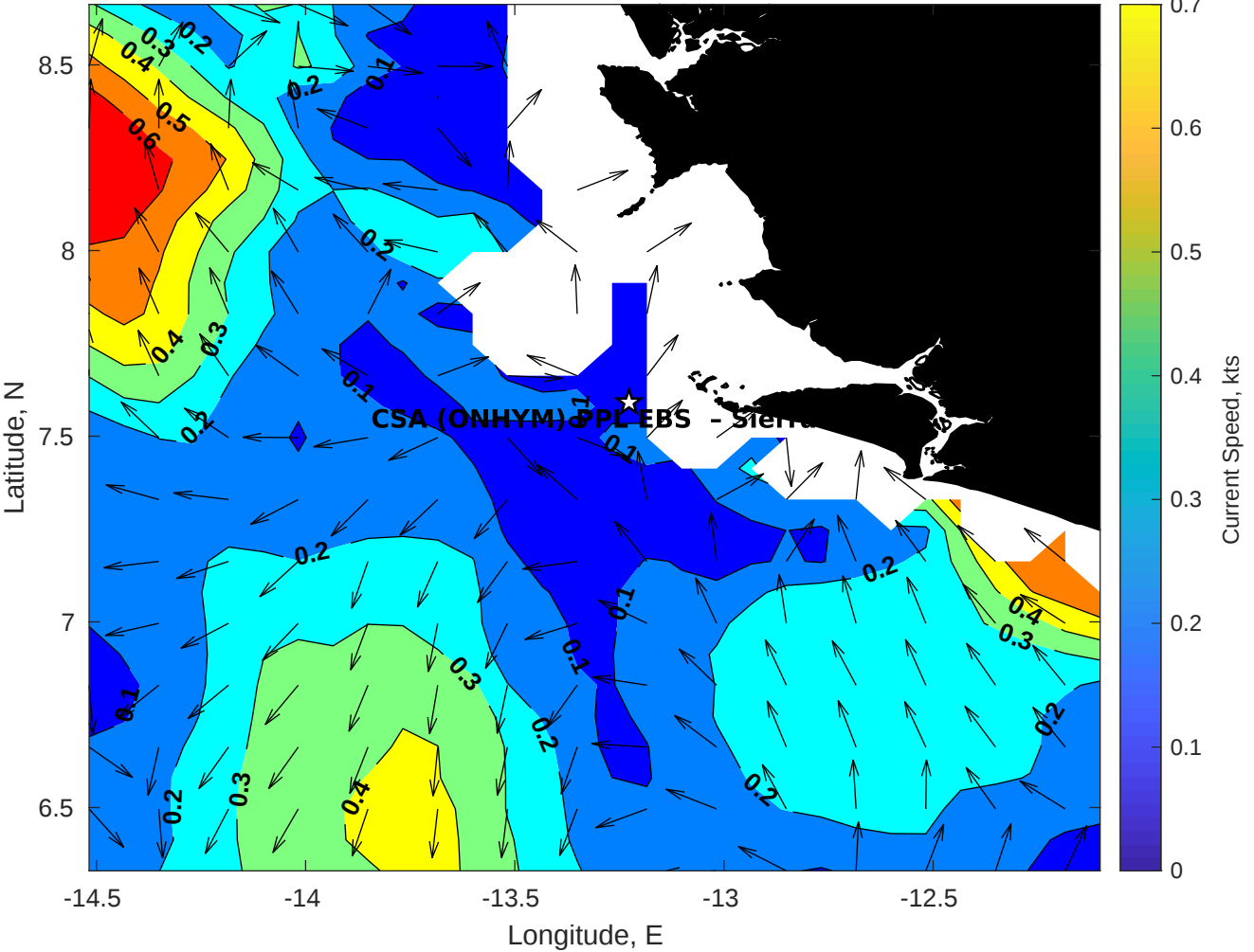
Surface Currents for CSA (ONHYM) PPL EBS - Sierra Leone at 28-Nov-2025 00:00:00
