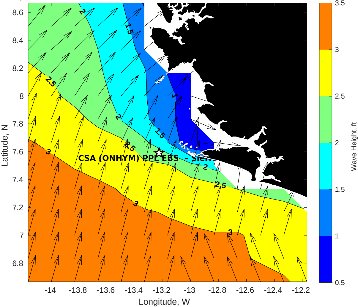
GFS Wave Height (ft) for CSA (ONHYM) PPL EBS - Sierra Leone at 29-Nov-2025 09:00:00
