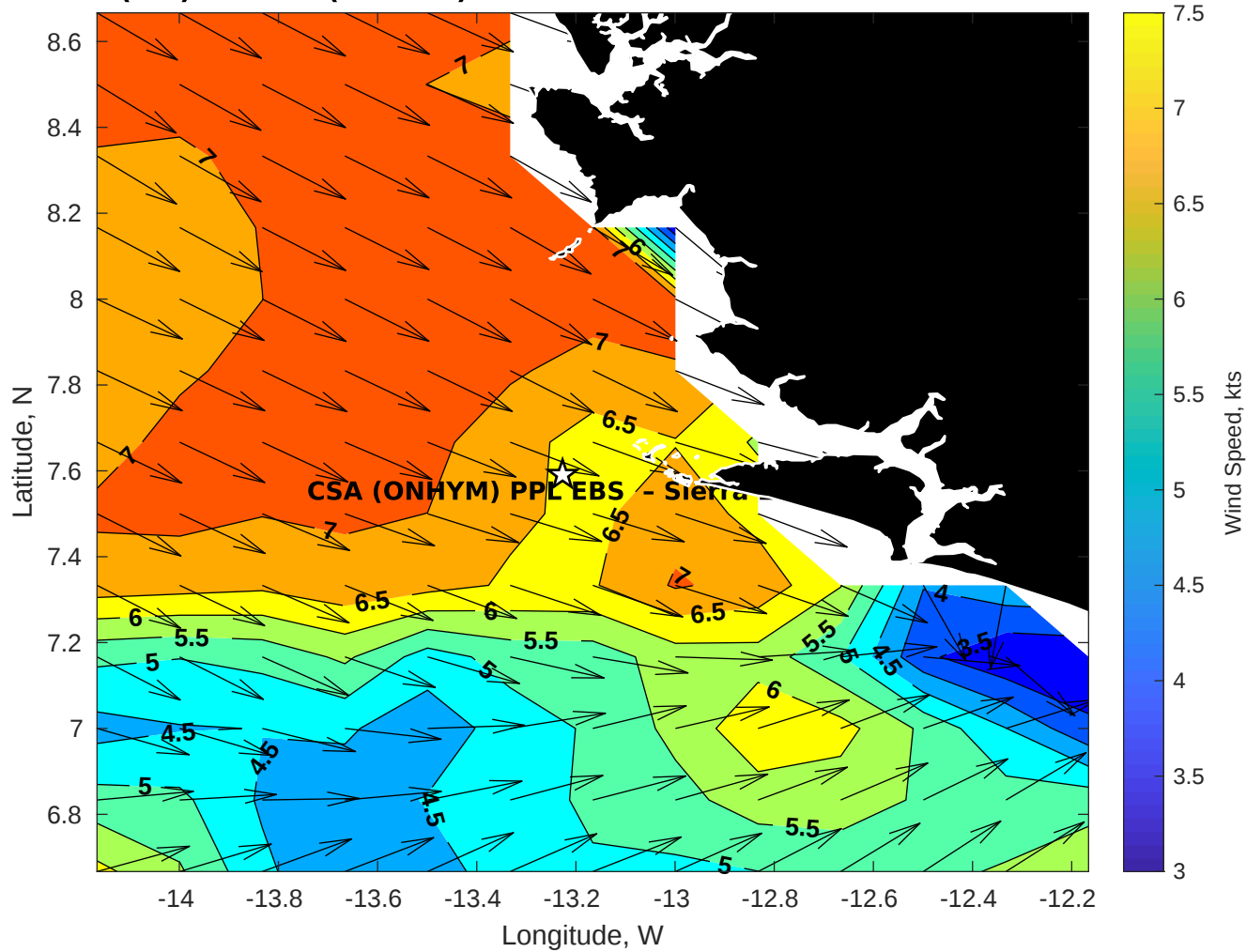
GFS Winds (kts) for CSA (ONHYM) PPL EBS - Sierra Leone at 29-Nov-2025 09:00:00
