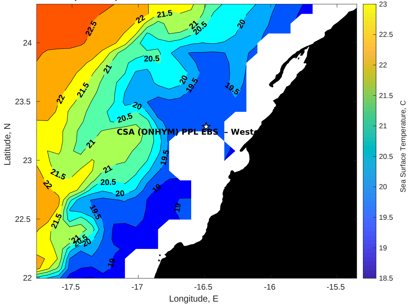
SST for CSA (ONHYM) PPL EBS - Western Sahara at 28-Nov-2025 00:00:00
